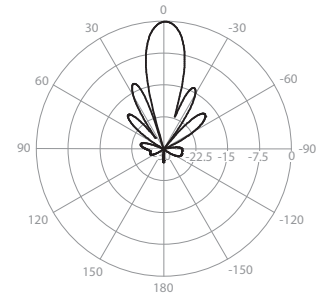
Elevation Pattern H
