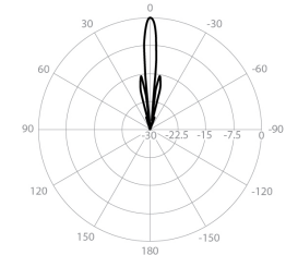
H - Port Pattern Elevation 5.6 GHz
