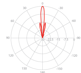
V - Port Pattern Elevation 5.6 GHz
